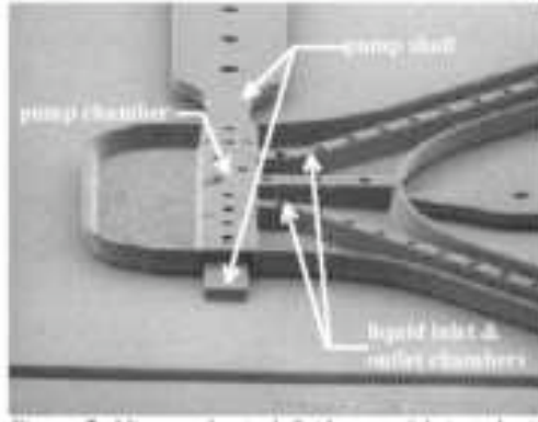
Figure 2. Micromechanical fluidic pump fabricated using with CMP.
